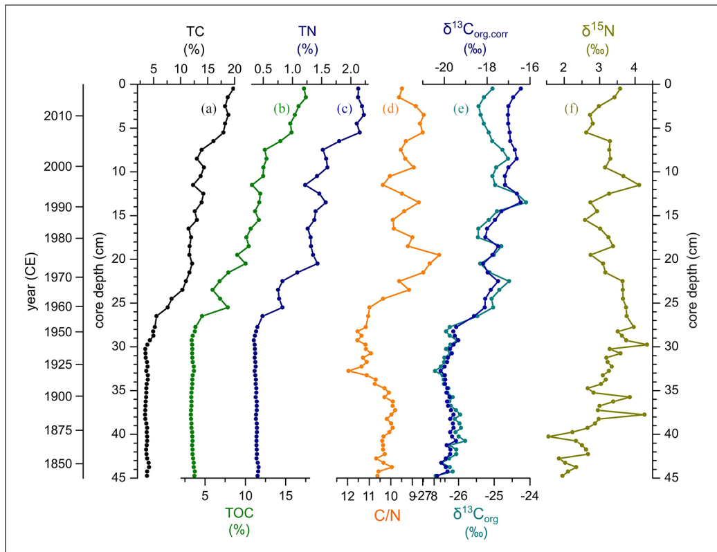
Figure 5. Depth profiles of TC (a), TOC (b), and TN (c) contents, C/N ((d) reversed plotted), \delta^{13}\text{C}_{\text{org,corr}} (e), and \delta^{15}\text{N} (f) in core EMB201/7-4.
