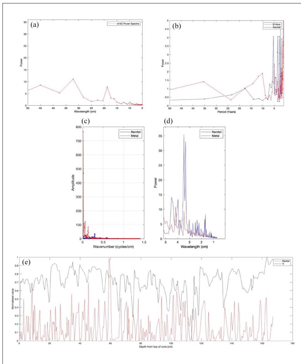
Figure 3. (a) Time series power spectra of \delta^{13}\text{C} analyses from the sediment core, (b) combined time series spectra for observed monthly rainfall and El Niño events, (c) spectra and plot of rainfall and heavy metal data used in construction of the depth to time conversion for the top 167 cm of the core, (d) comparison of the spectra of the heavy metal and rainfall measurements with depth, after adjusting the datasets using sediment load data for the San Francisco Estuary to account for variations in sediment flux, (e) comparison of the rainfall and subsampled heavy metal data (Ti) for the top 167 cm of the core (note: both datasets have been normalised to their maximum values to aid comparison). The dates of the peaks and troughs in the rainfall data are known, enabling a chronology for the core to be constructed. Further explanation of these analyses is presented in the main text and Supplemental File.
