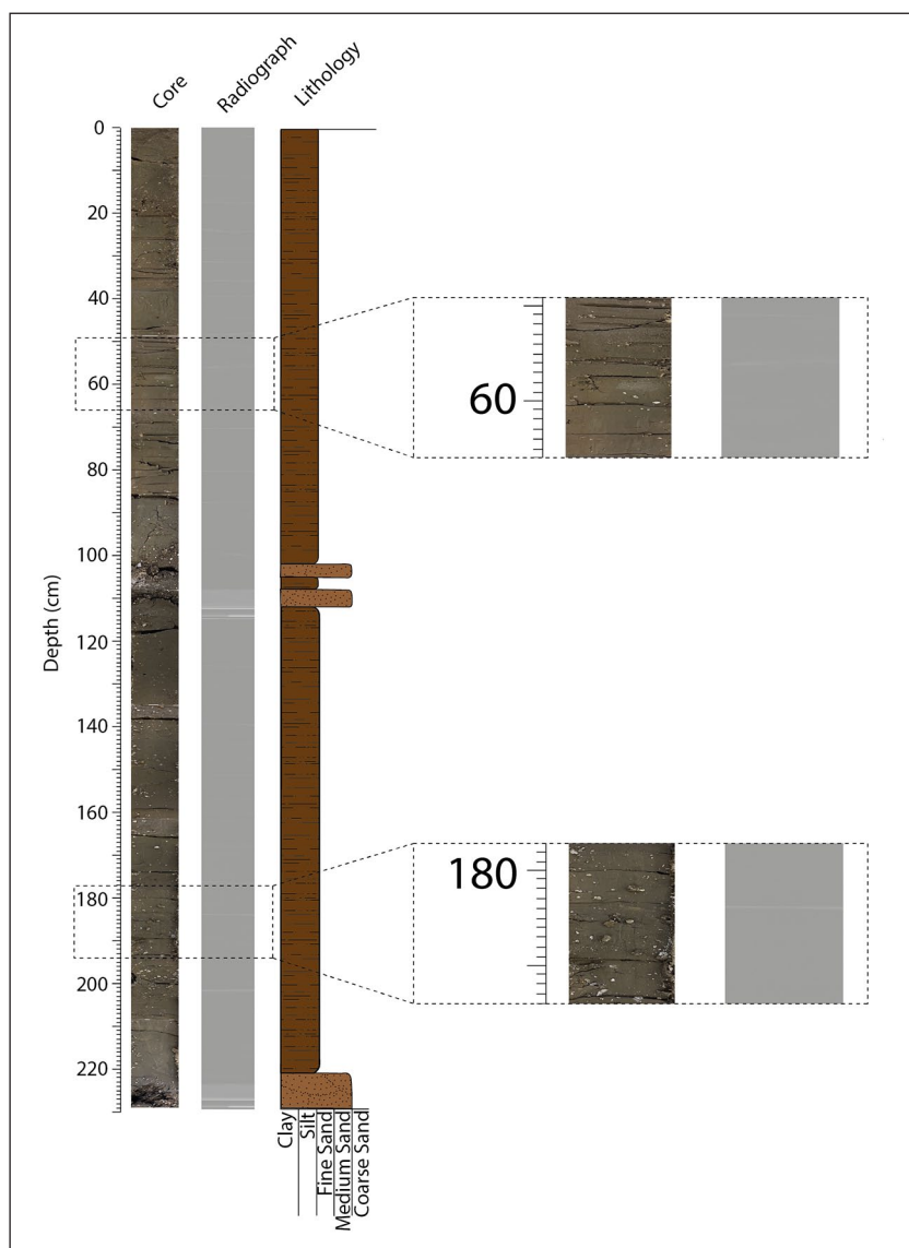
Figure 2. Sediment core image, lithology, and ltrax X-radiograph core scan of core SFB-20A. The cracks evident in the sediment core (left column) may align with lamination boundaries.
