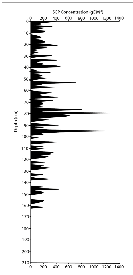
Figure 7. Downcore trends in the concentration of spheroidal carbonaceous particles (SCPs). The lowest occurrence of SCPs at 165 cm approximates 1967.
